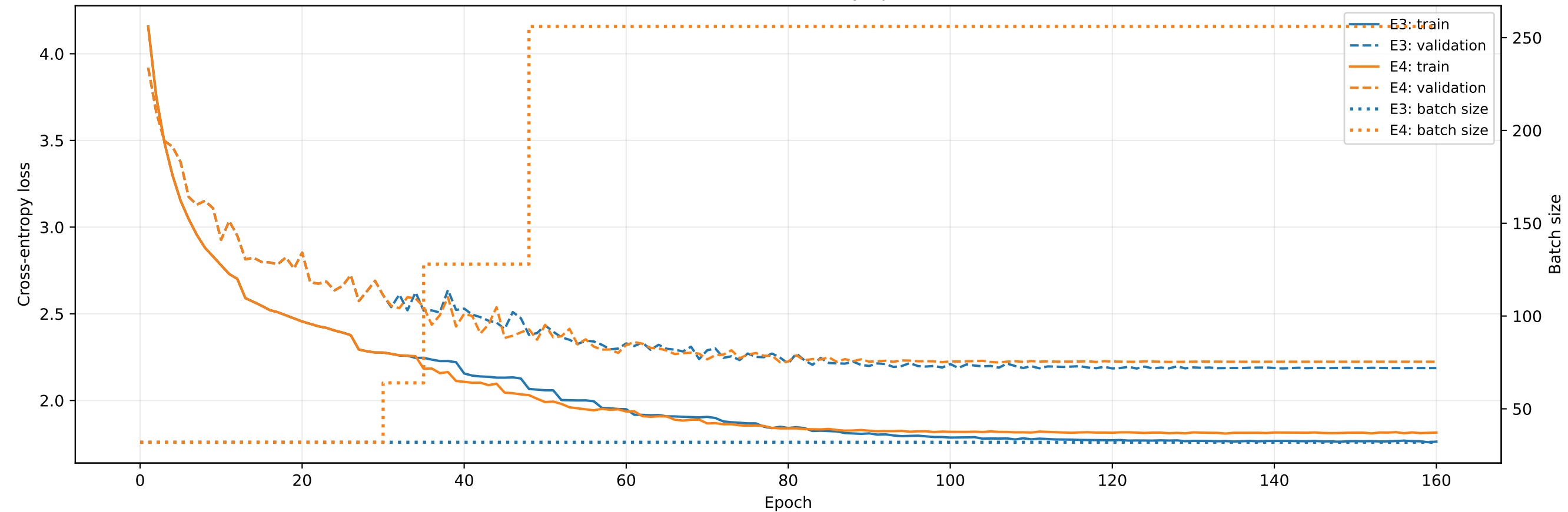
Loss and batch size by epoch
