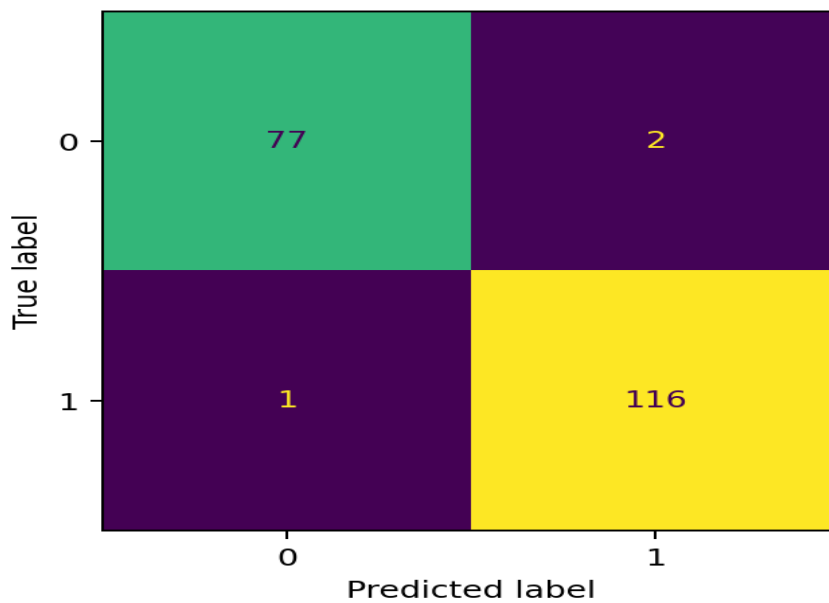
Purchase Intention Model — Confusion Matrix
