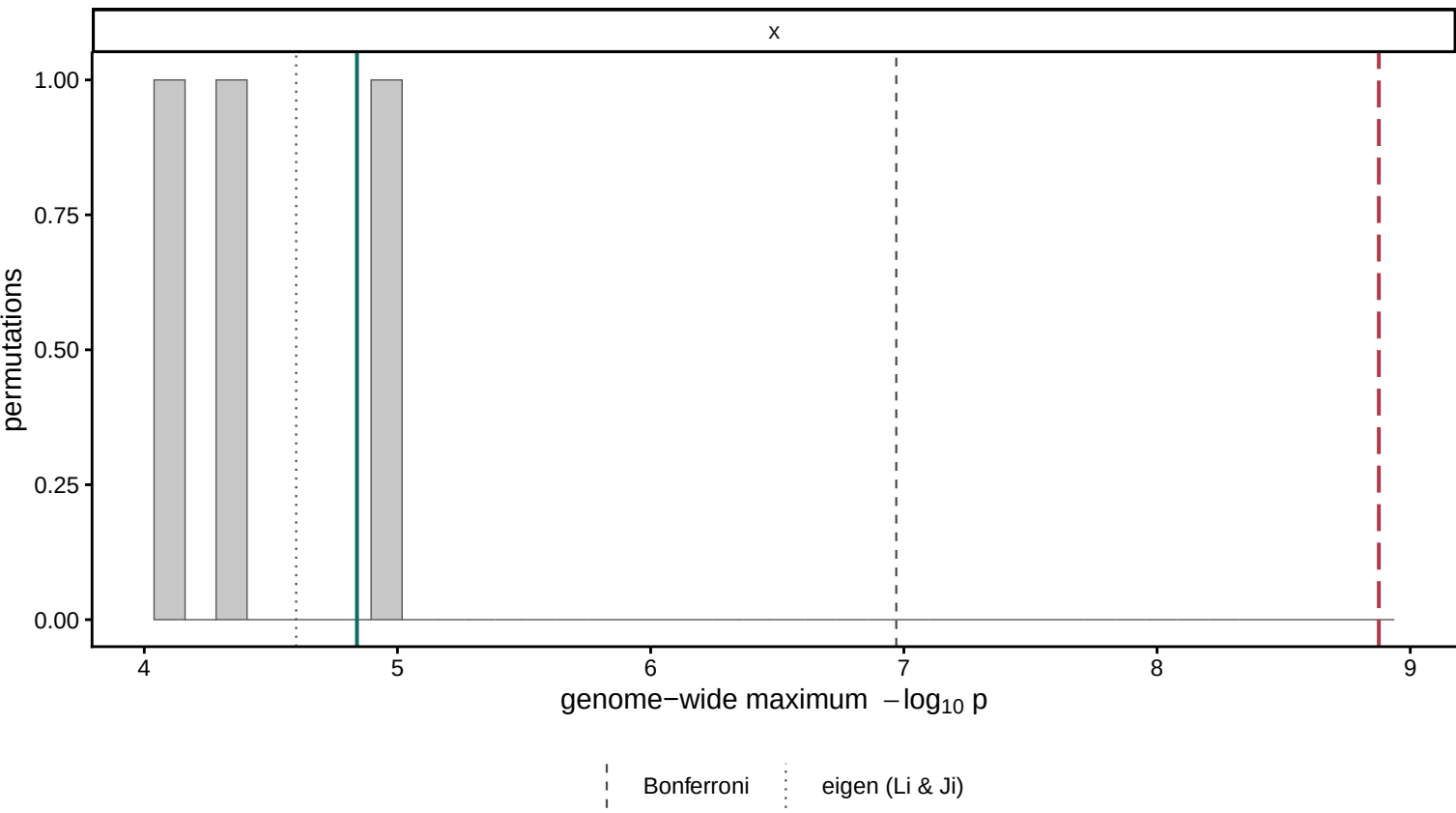
Permutation null for the genome-wide maximum teal = permutation threshold at alpha 0.05; red dashed = observed scan
