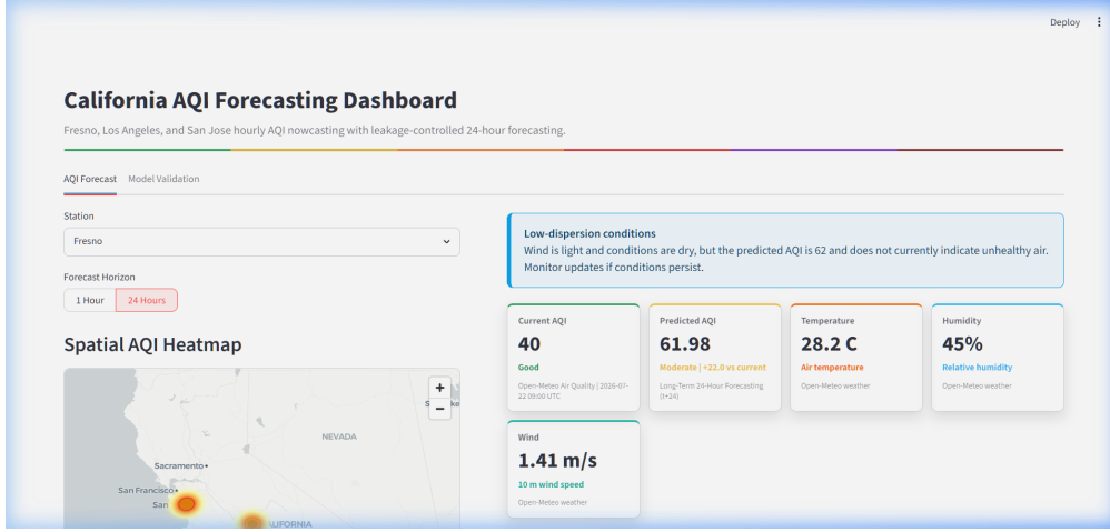
Fig. 6: Real-time early warning web application UI showing the PyDeck spatial AQI heatmap, atmospheric condition indicators, short-term and 24-hour prediction metrics, and automated alert panels.
