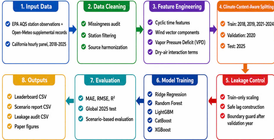
Fig. 4: AQI forecasting pipeline architecture.
