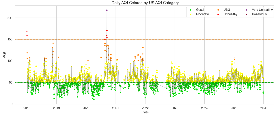
Fig. 7: Daily AQI observations colored by U.S. AQI health category.
