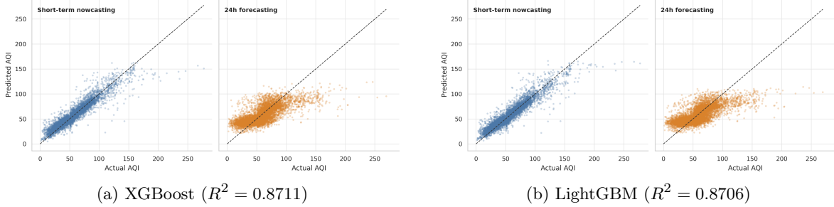
Fig. 8: Predicted versus actual AQI scatter diagnostics on the independent 2025 test year for top-performing gradient boosted decision tree regressors.
