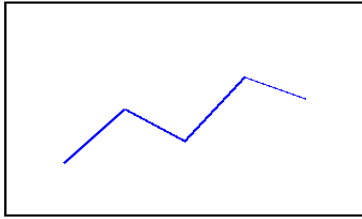
Chart 7: Performance Metrics
