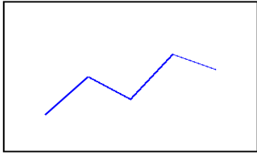
Chart 1: Performance Metrics
