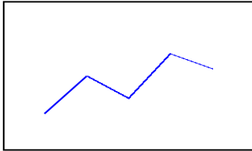
Chart 11: Performance Metrics
