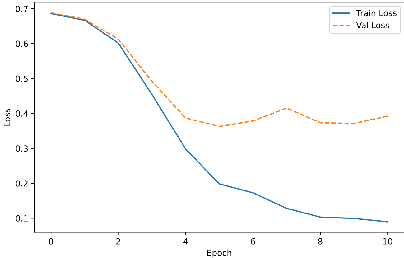
MLP Loss Curve
