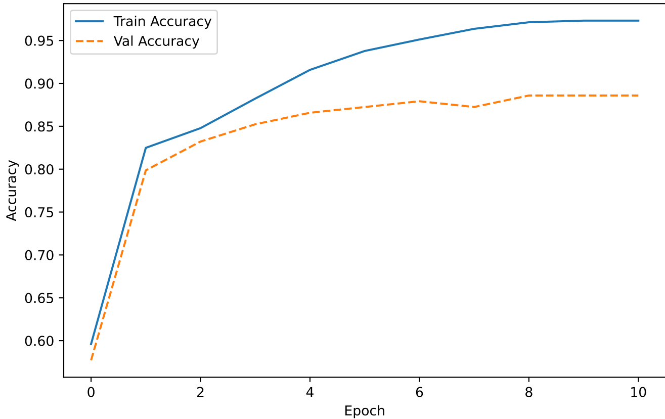
MLP Accuracy Curve
