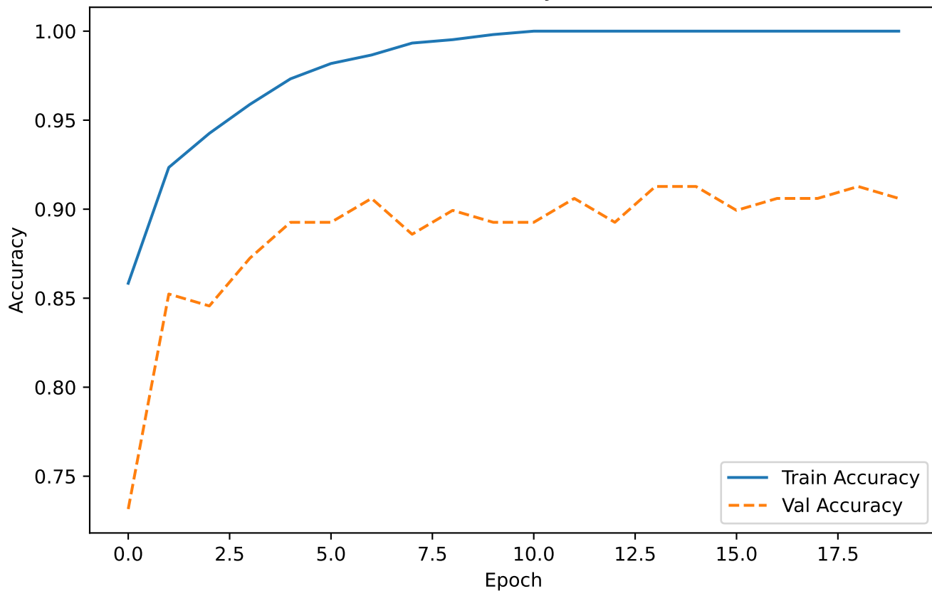
CNN Accuracy Curve
