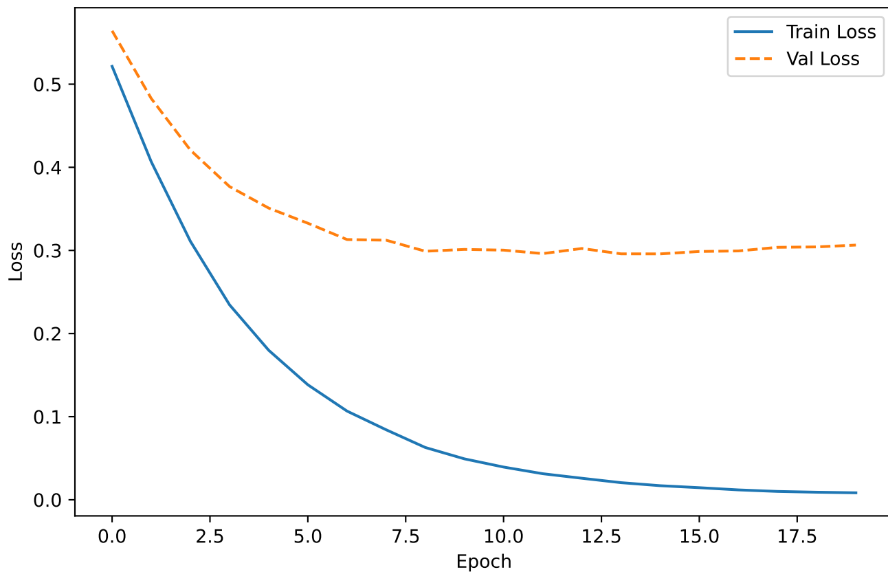
CNN Loss Curve
