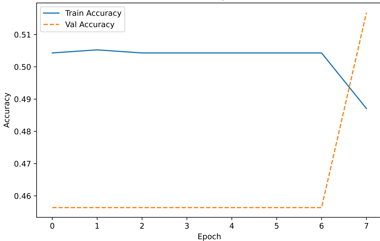
RNN Accuracy Curve
