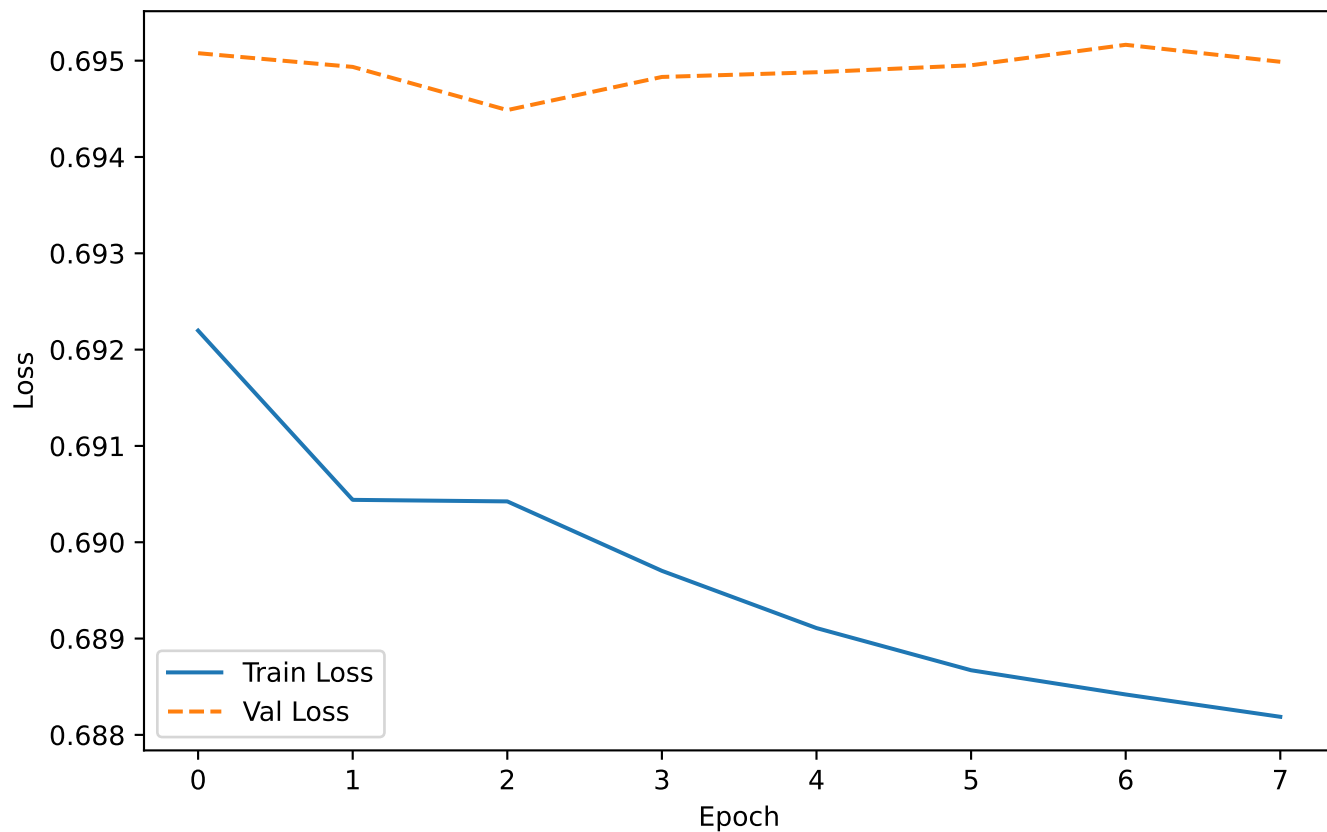
RNN Loss Curve
