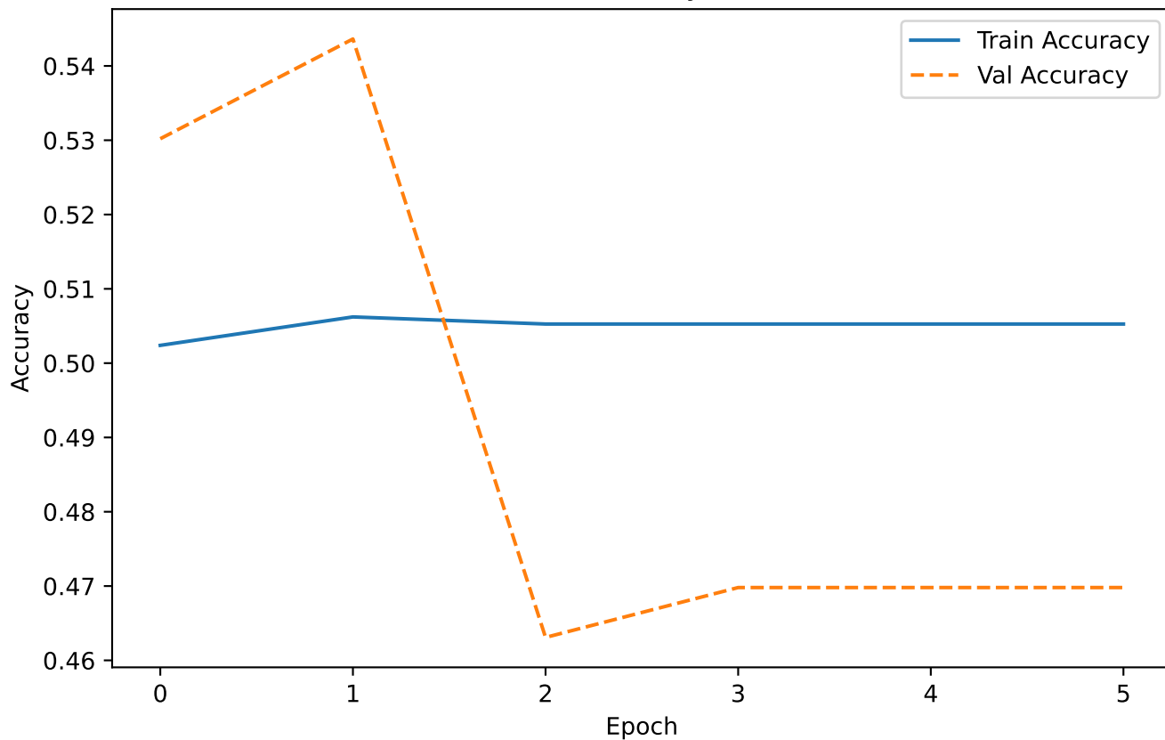
LSTM Accuracy Curve
