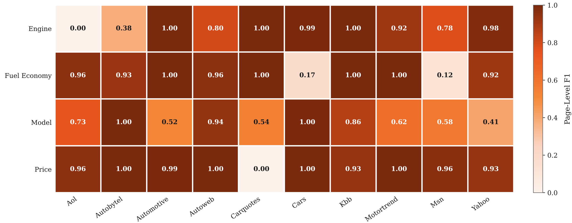
SWDE Auto: Page-Level F1 by Website and Attribute
