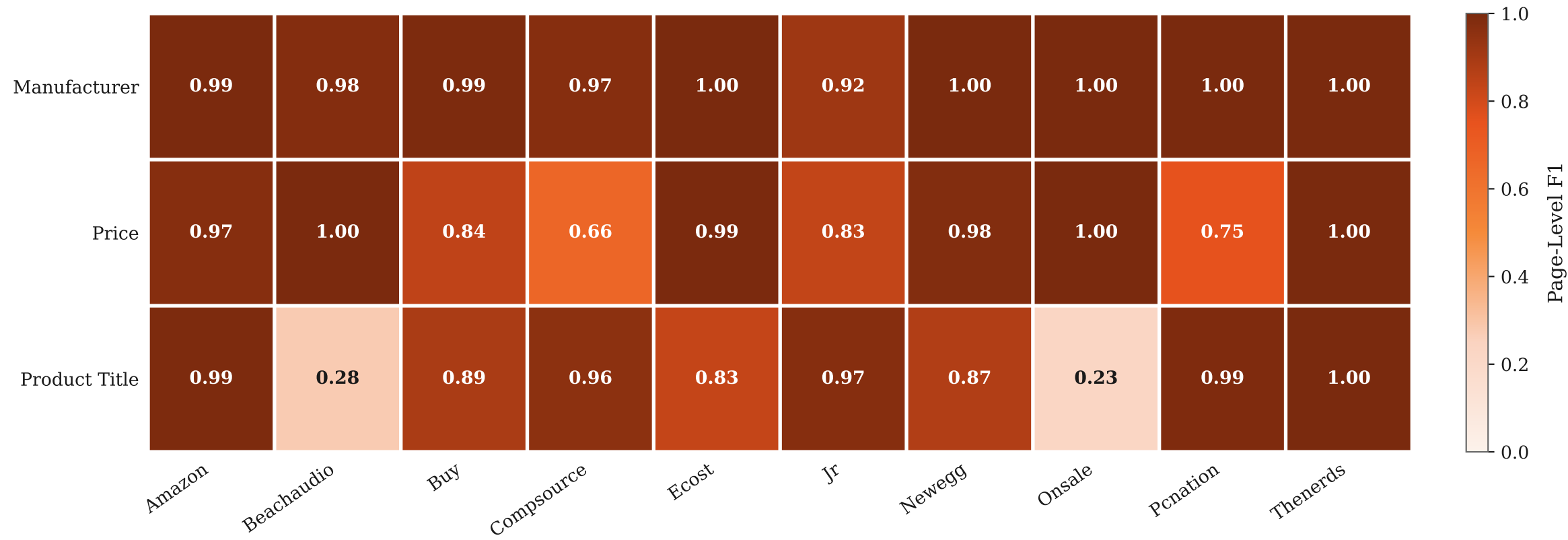
SWDE Camera: Page-Level F1 by Website and Attribute
