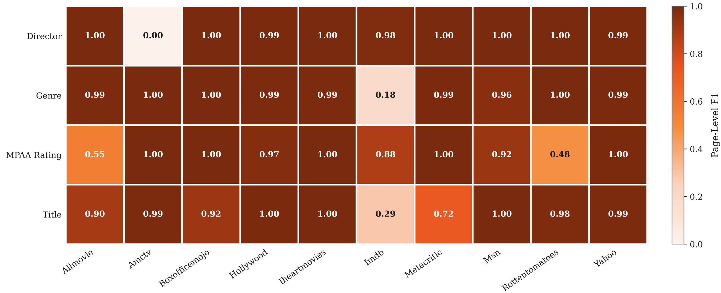
SWDE Movie: Page-Level F1 by Website and Attribute
