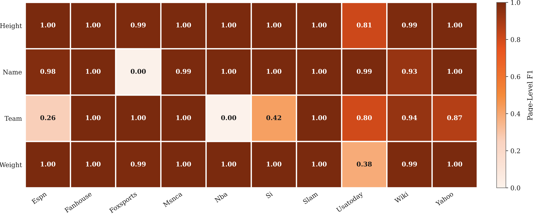
SWDE NBA Player: Page-Level F1 by Website and Attribute
