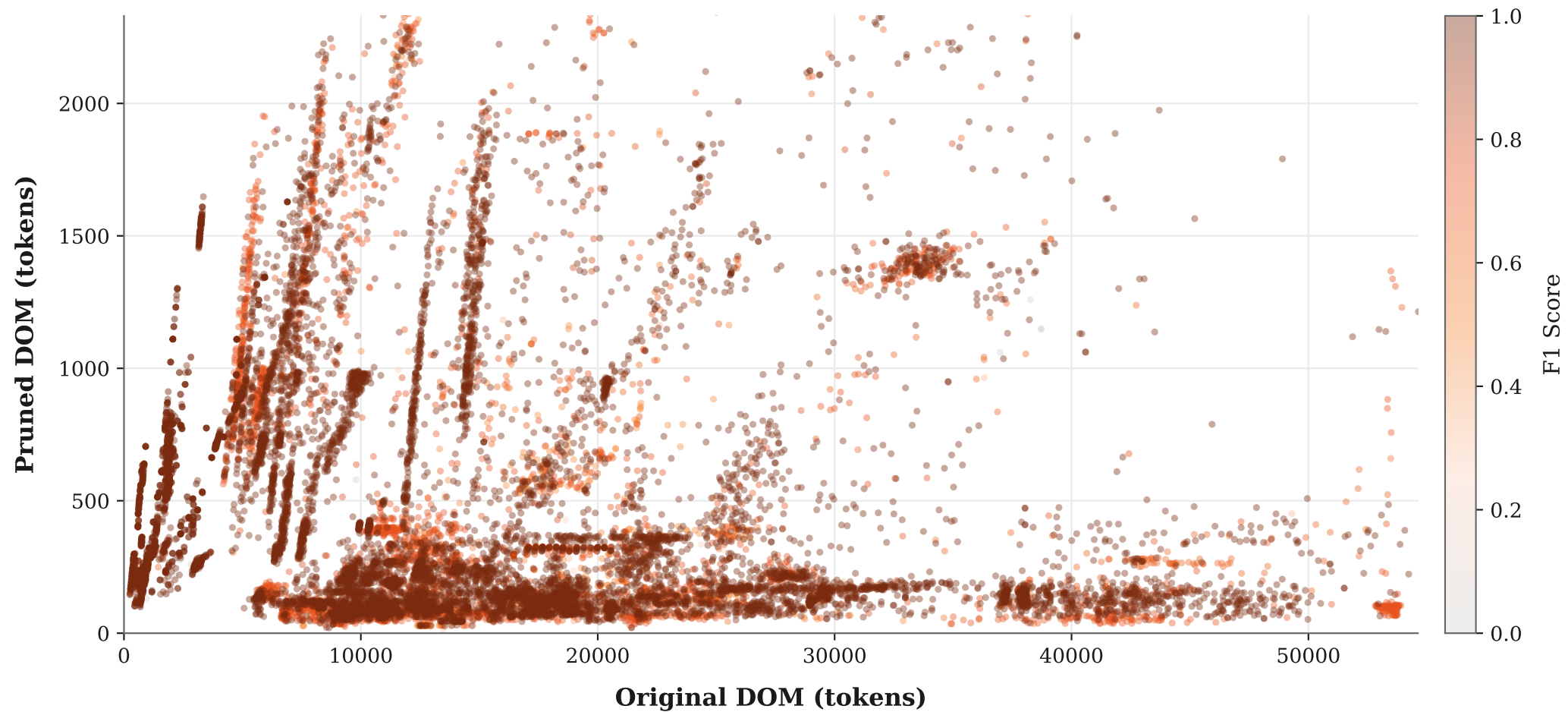
DOM Reduction: Original vs. Pruned Tokens
