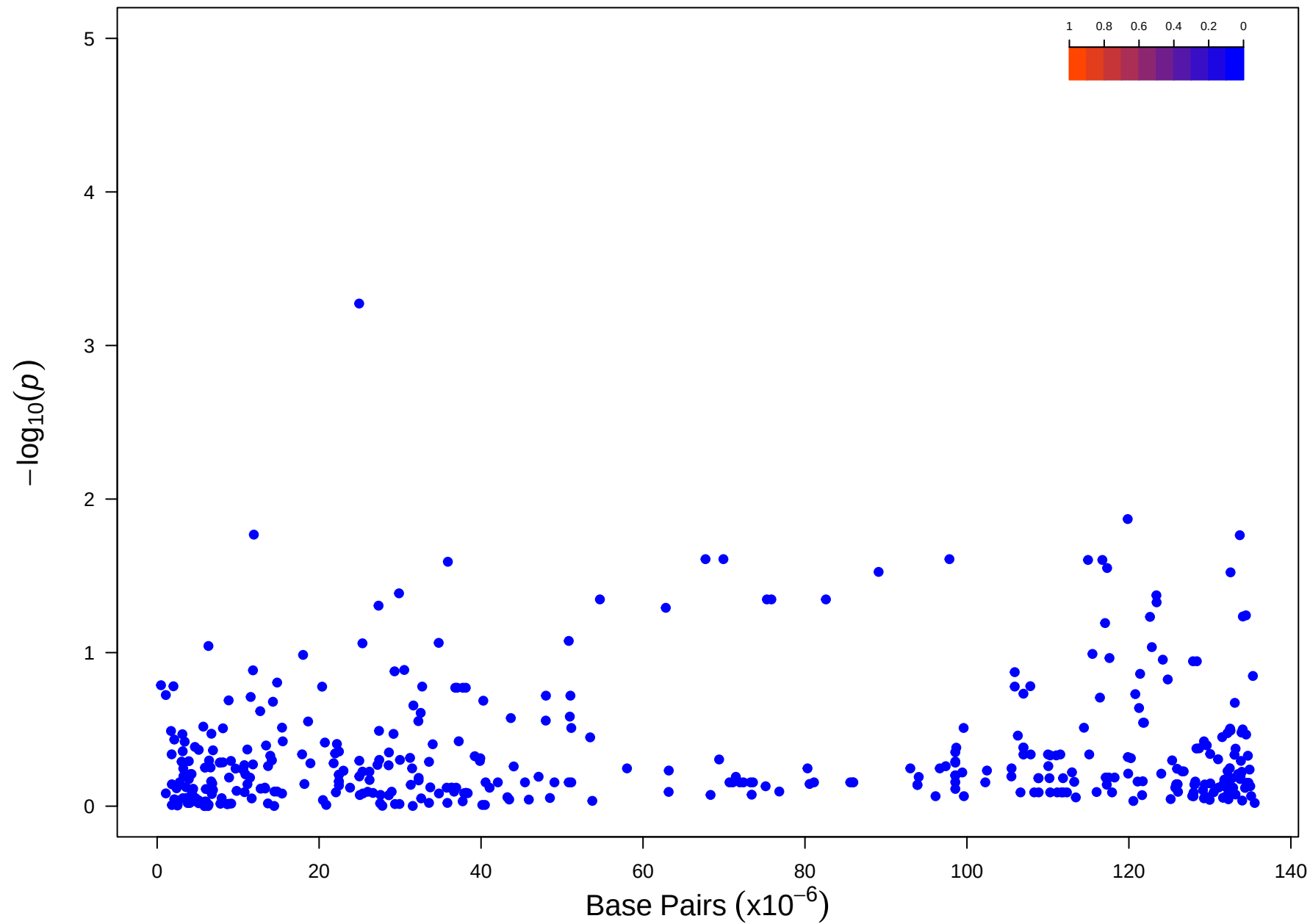
Chromosome 13
