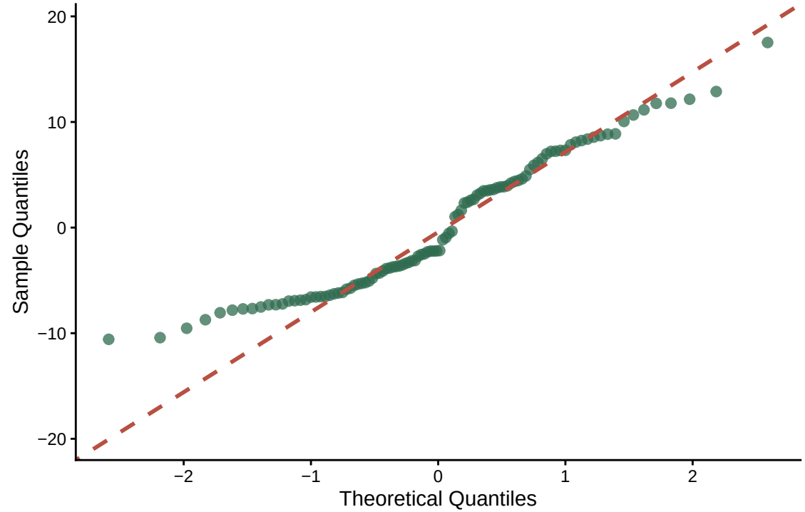
Q-Q Plot (BLUPs)
