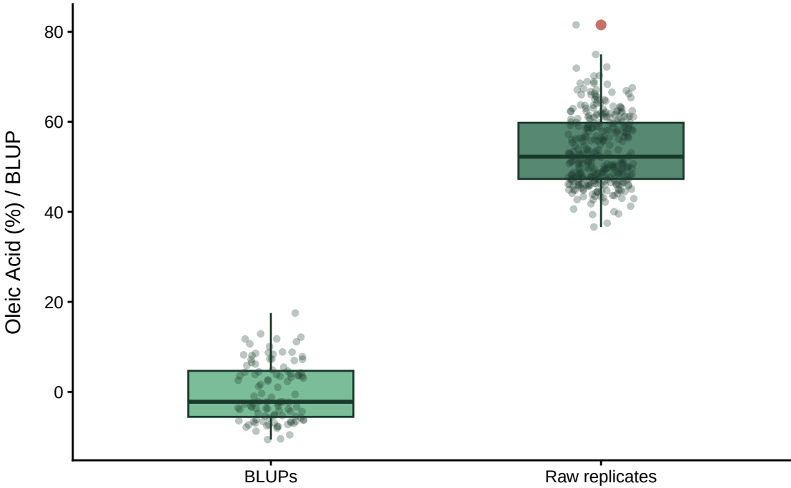
Raw vs BLUPs
