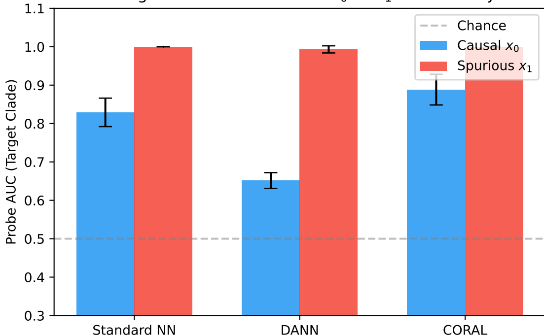
Design-Oracle Latent Probe: x_0 vs x_1 Decodability
