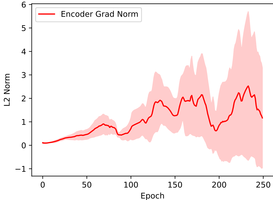
Gradient Norms ( \lambda = 1.0 )
