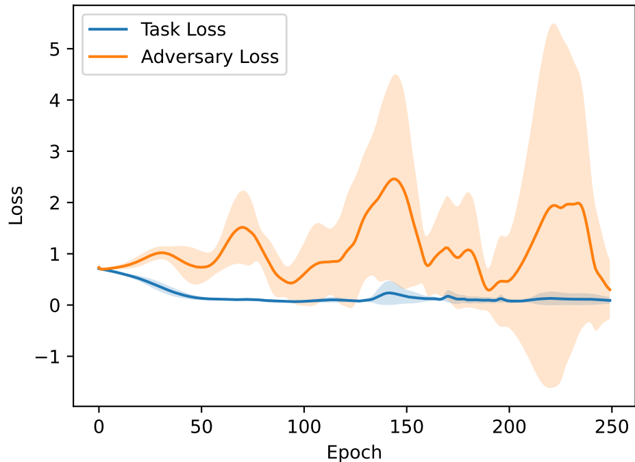
Loss Trajectories ( \lambda = 1.0 )
