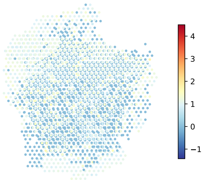
Gene 178 — Observed
