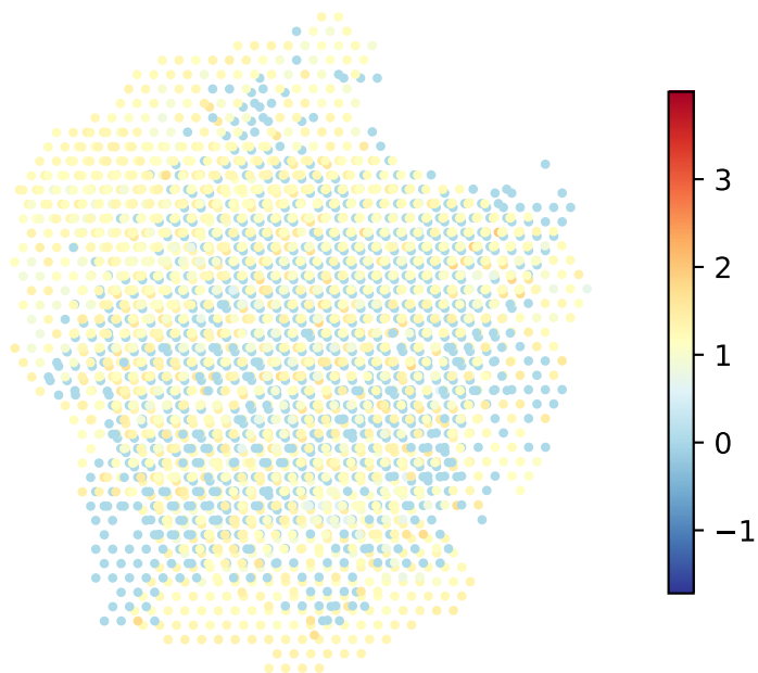
Gene 244 — Observed
