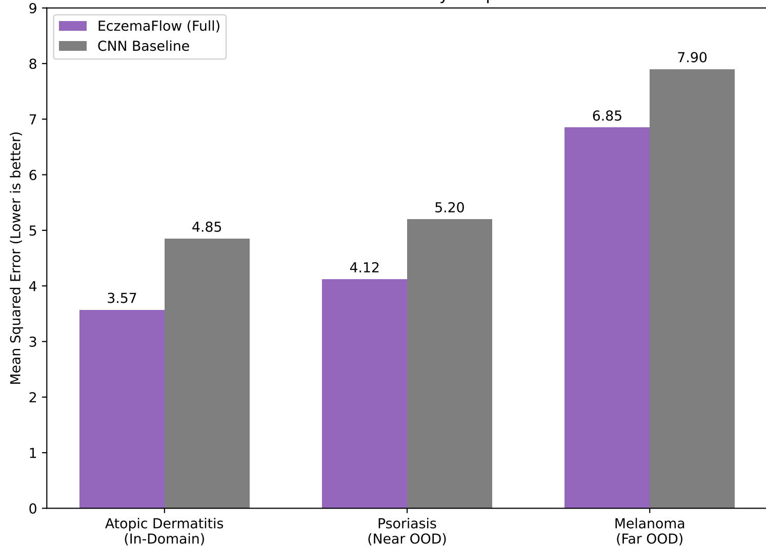
Cross-Disease Generalizability of Spatial Inference
