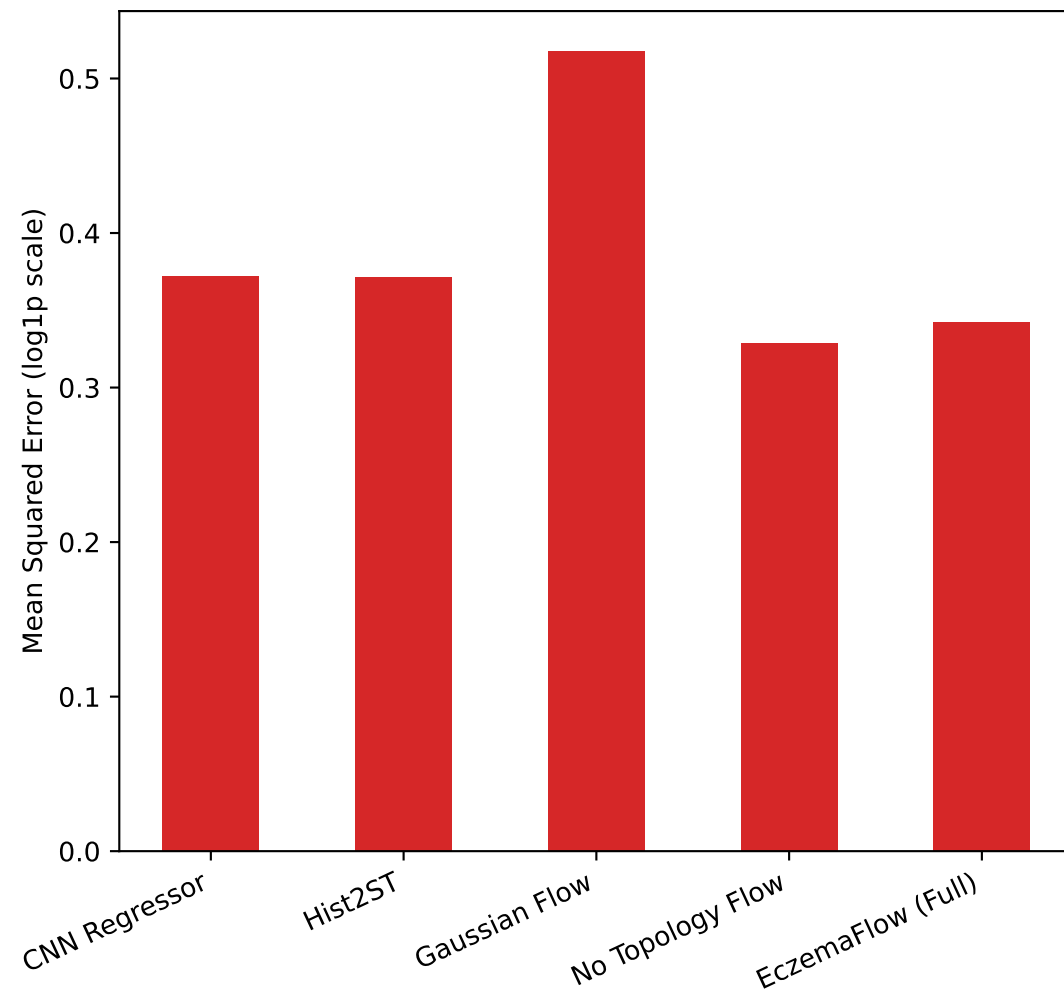
MSE Performance
