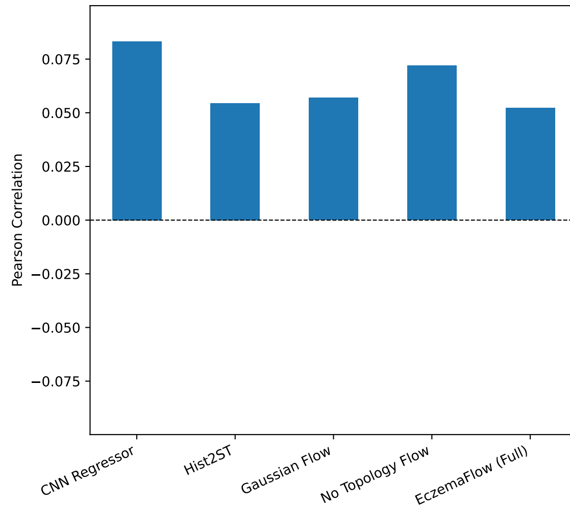
PCC Performance
