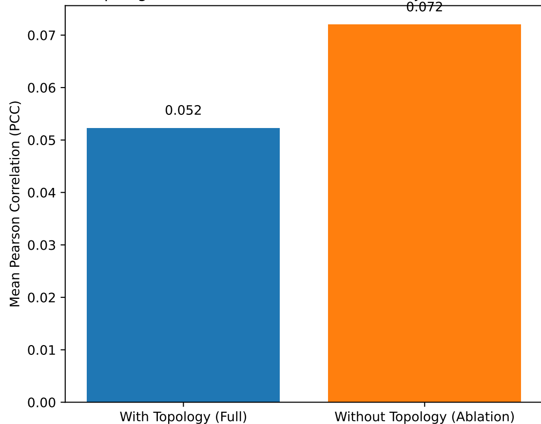
Topological Feature Extractor Ablation (Rejection of H1)
