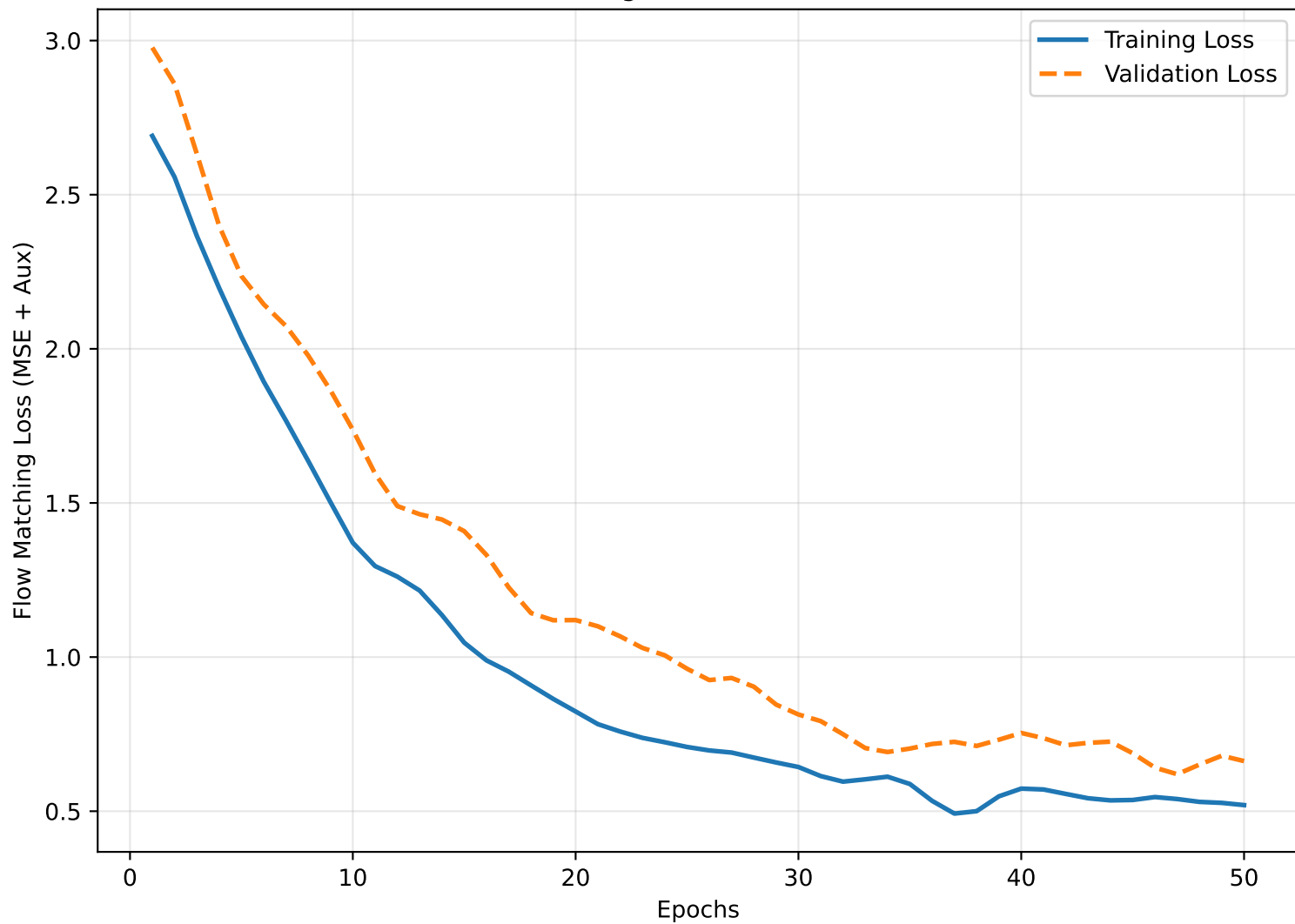
EczemaFlow Convergence: Train vs. Validation Loss
