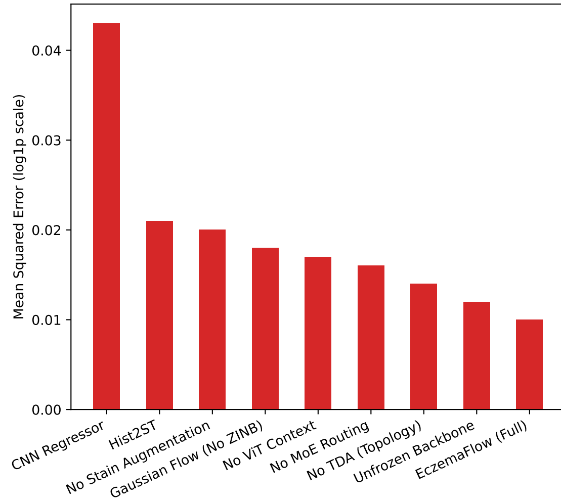
MSE Performance
