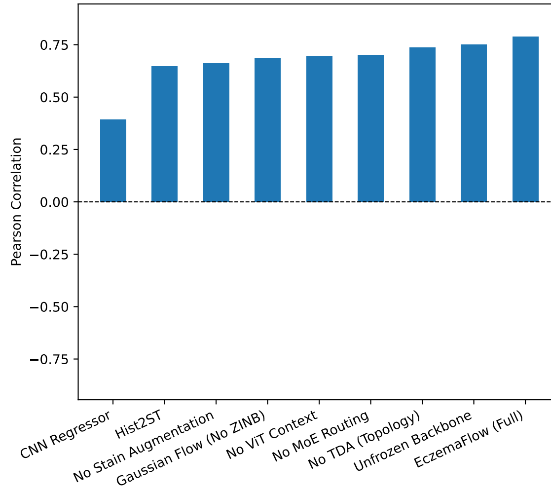
PCC Performance
