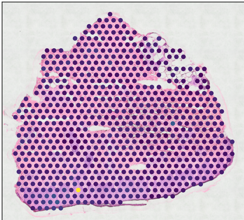
Ground Truth Total UMI Counts
