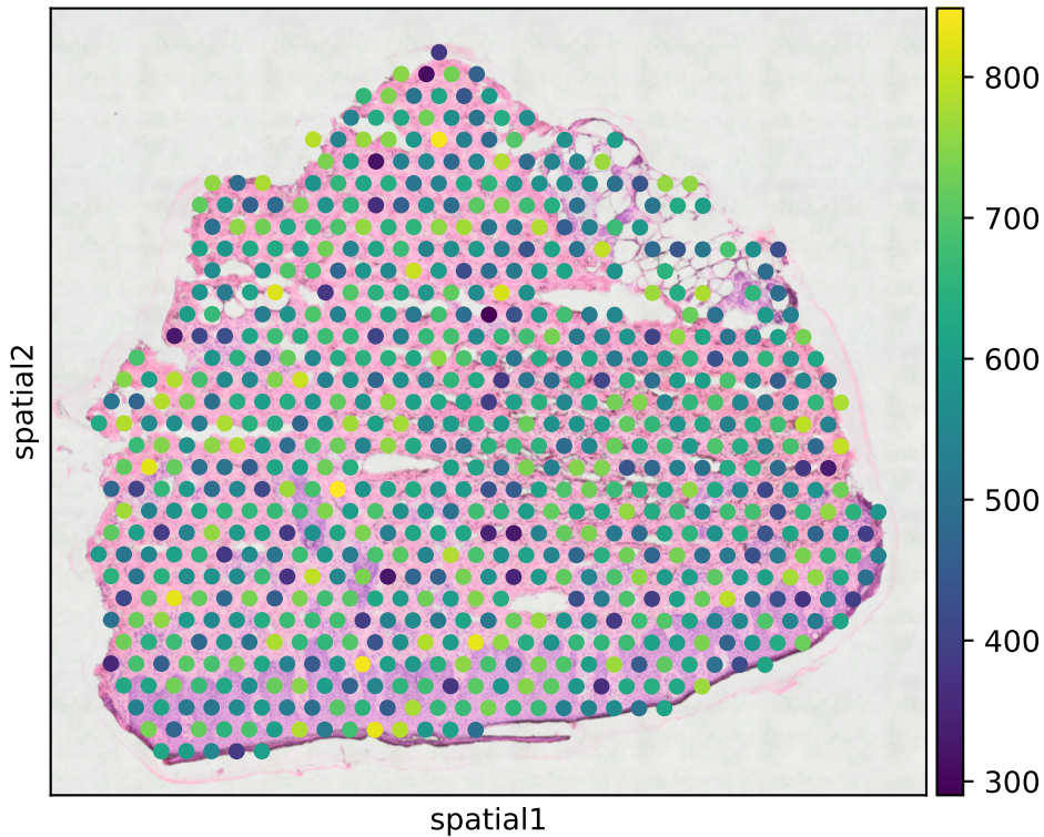
Predicted Total UMI Counts
