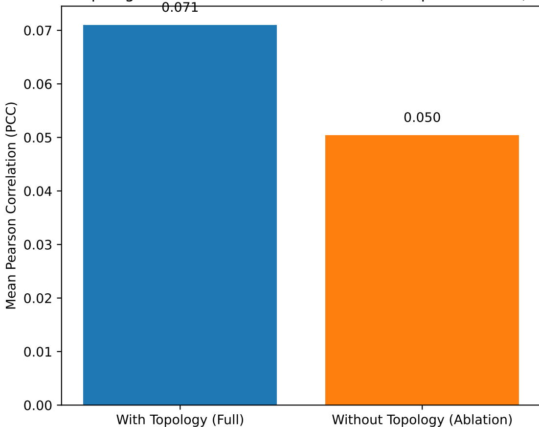
Topological Feature Extractor Ablation (Acceptance of H1)
