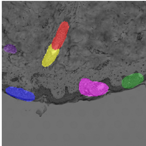
StarDist Segmentation
