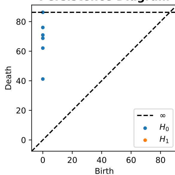
Persistence Diagram
