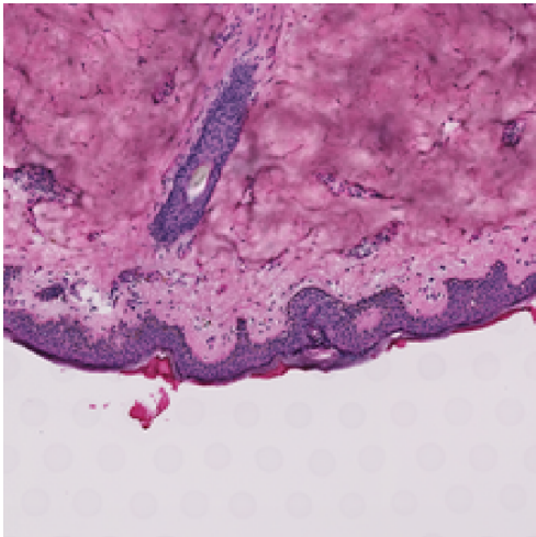
H&E Patch
