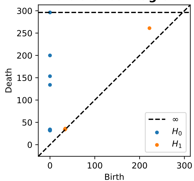
Persistence Diagram
