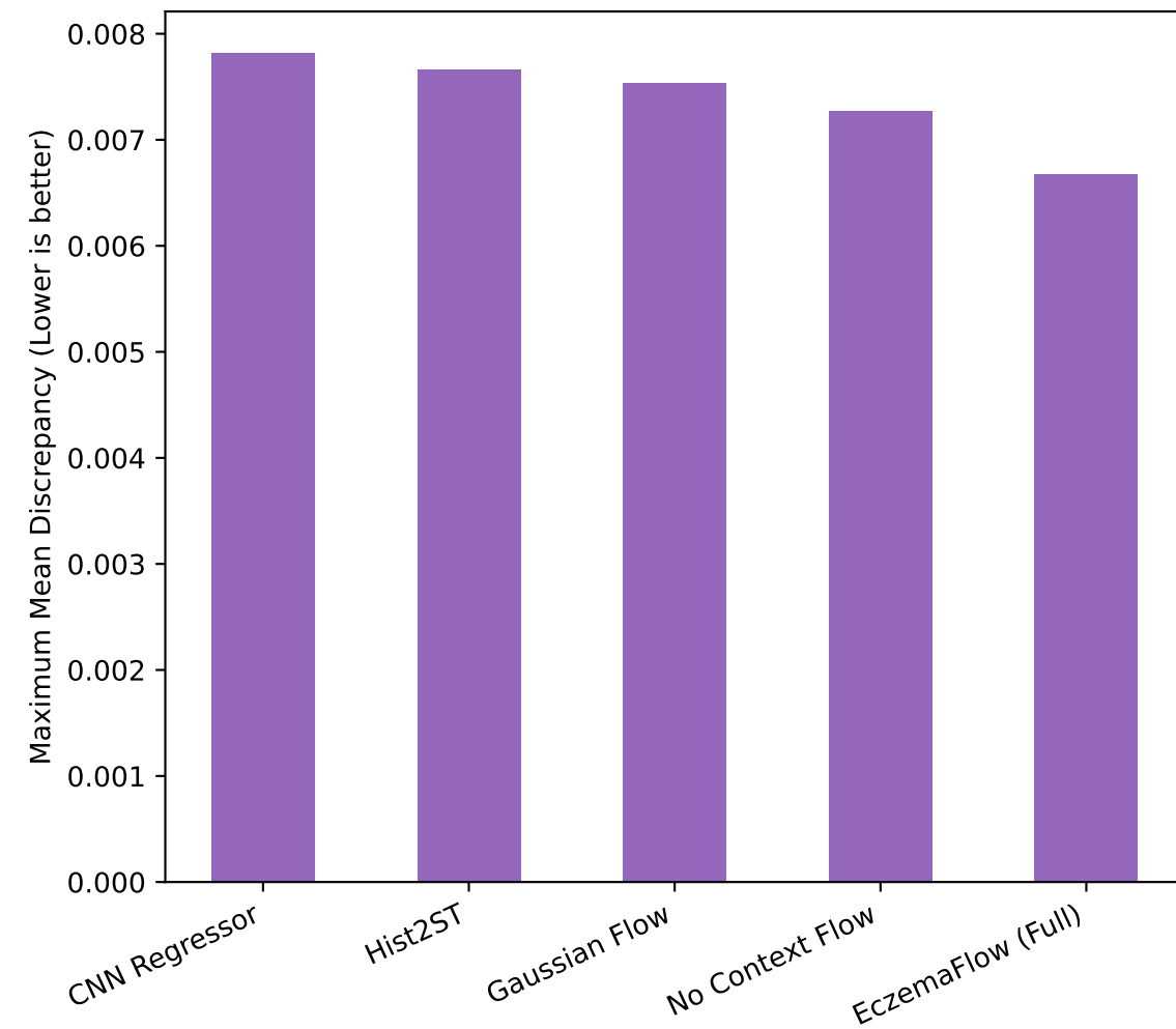
Generative Calibration (MMD)
