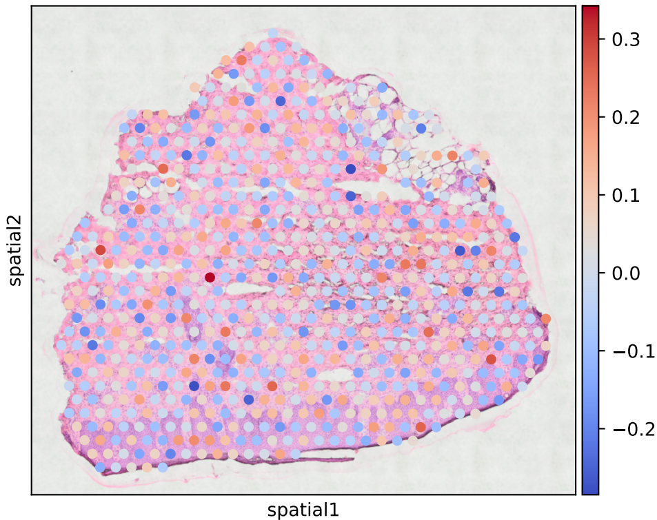
KRT14 (Residual)
