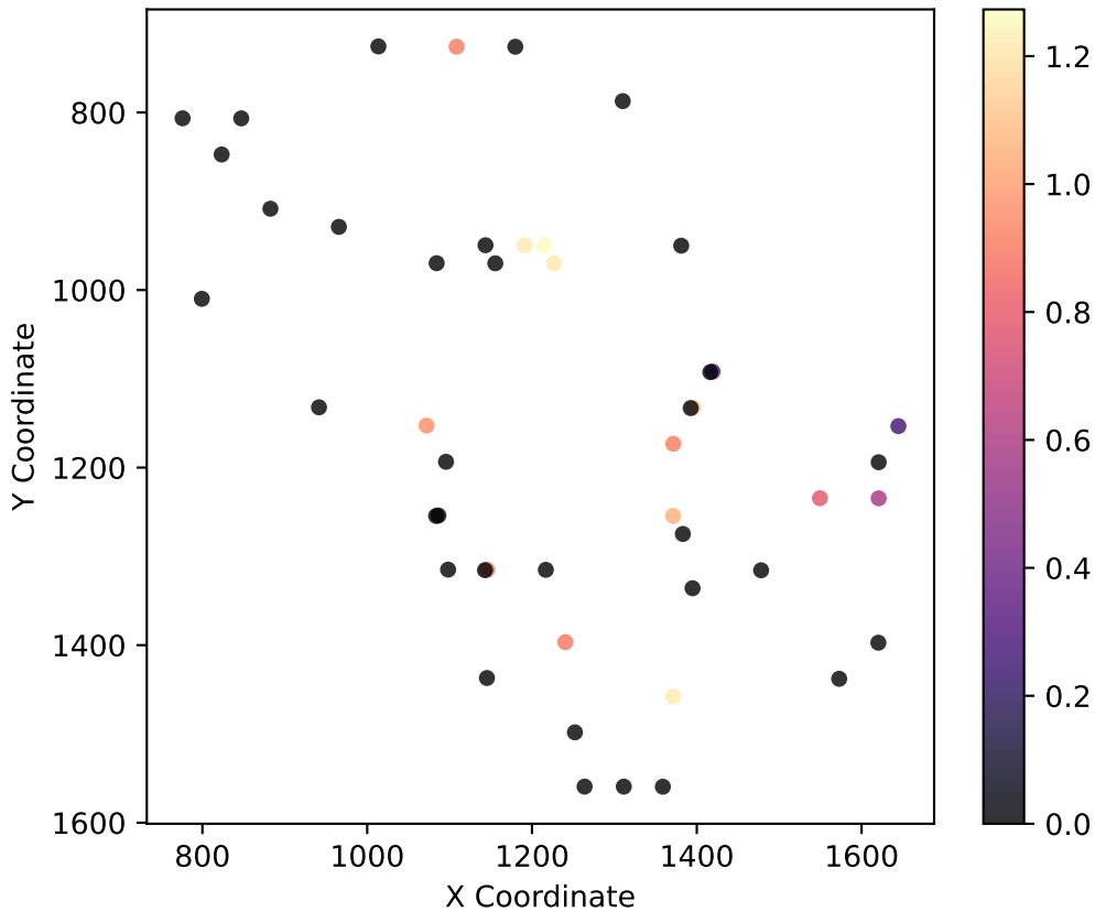
Ground Truth COL18A1 Spatial Expression
