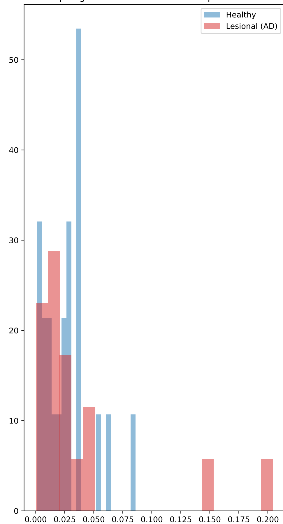
Topological Invariants: Betti-1 Loop Lifetimes
