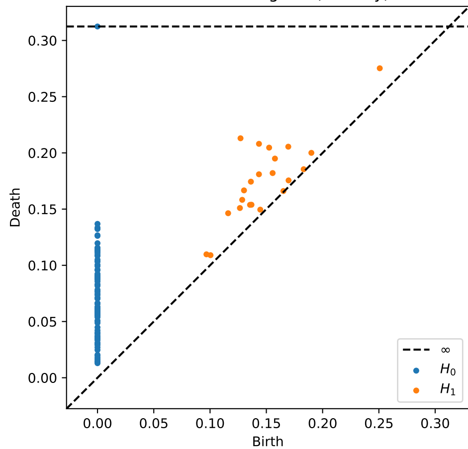
Persistence Diagram (Healthy)
