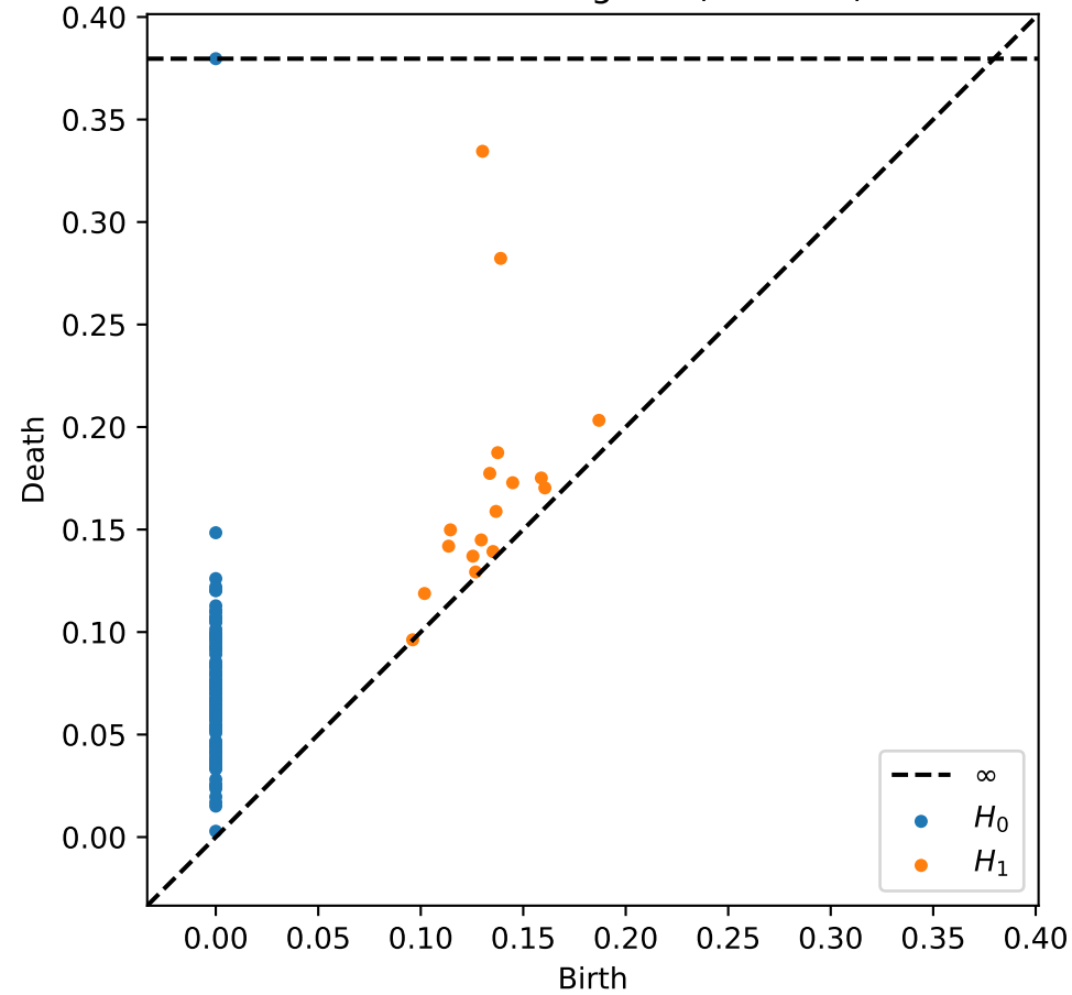
Persistence Diagram (Lesional)
