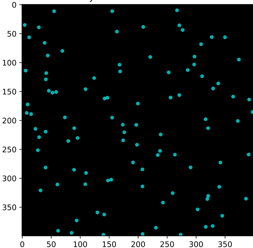
Persistence Diagram (Healthy)
