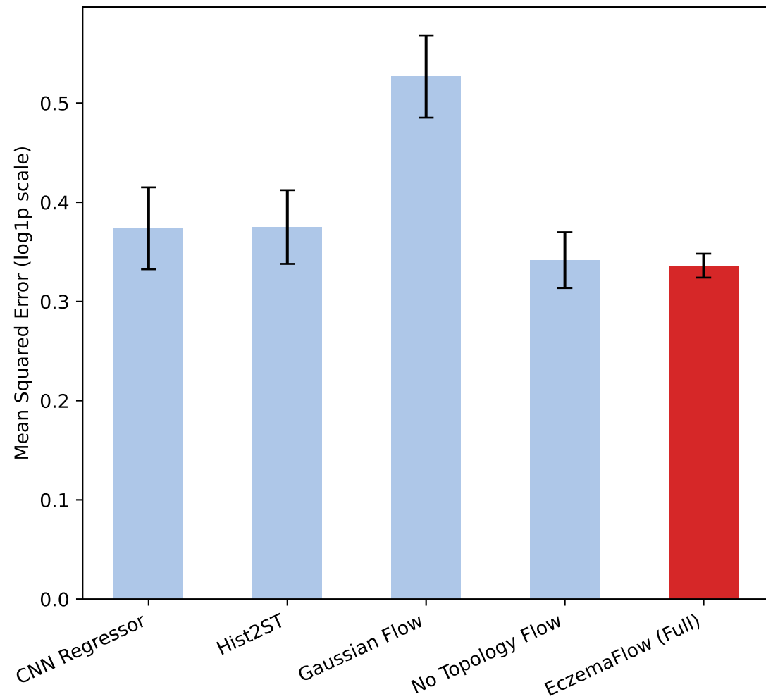
MSE Performance (6-fold LOOCV, \pm 95\% CI)
