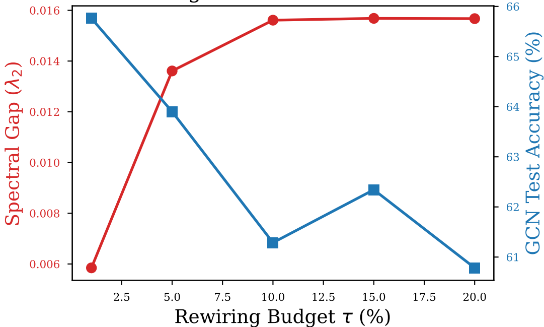
The Budget Trade-Off on CiteSeer
