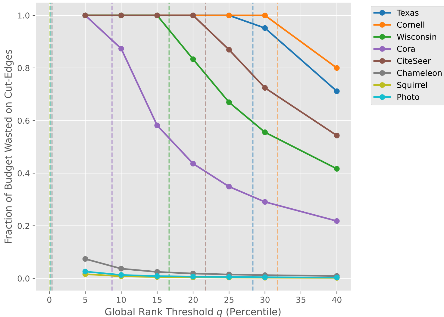
Empirical q -Sweep: Cut-Edge Saturation Across 8 Datasets
