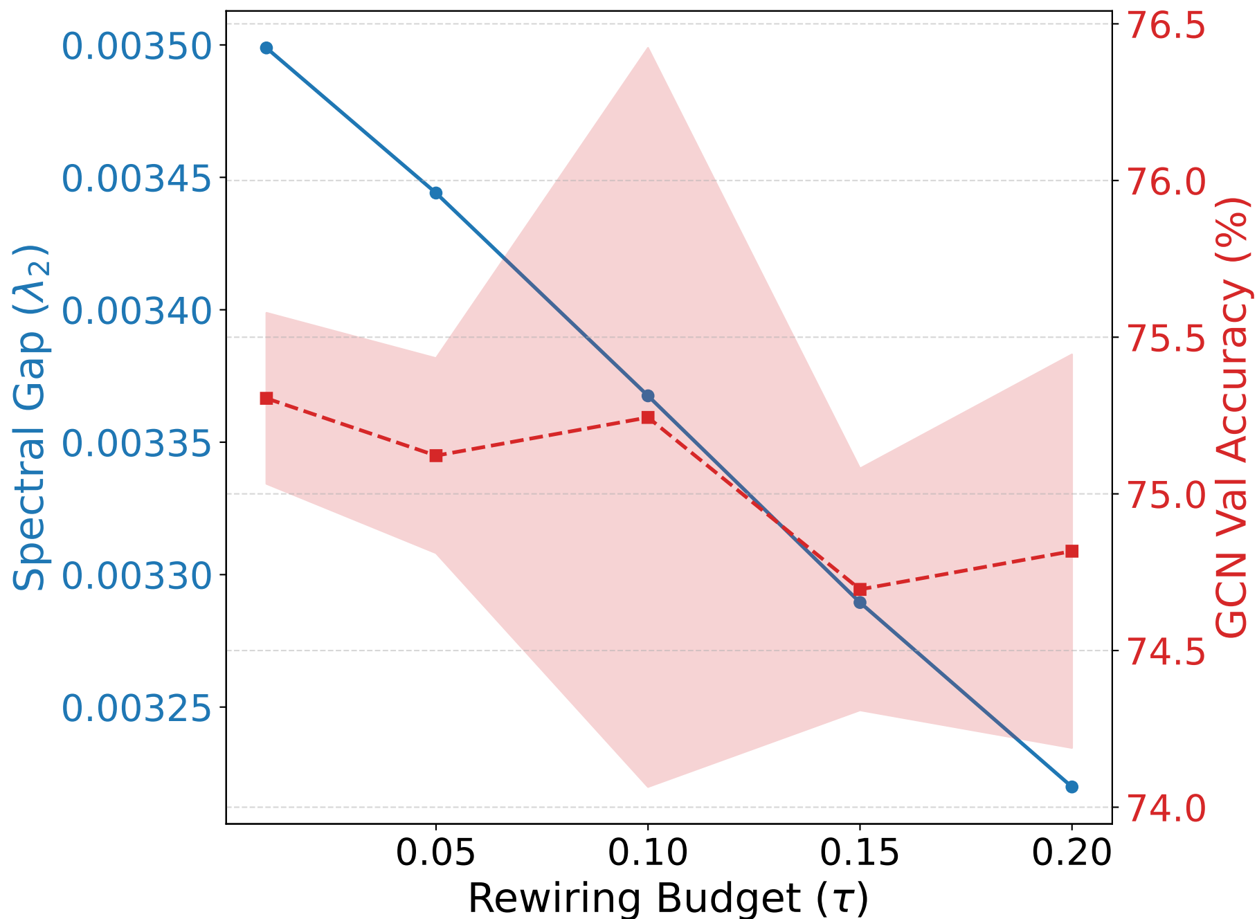
Effect of Rewiring Budget ( \tau ) on Spectral Gap & Accuracy
