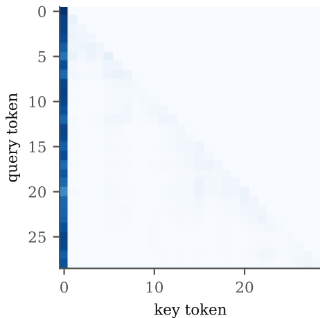
layer 21: head-averaged attention
