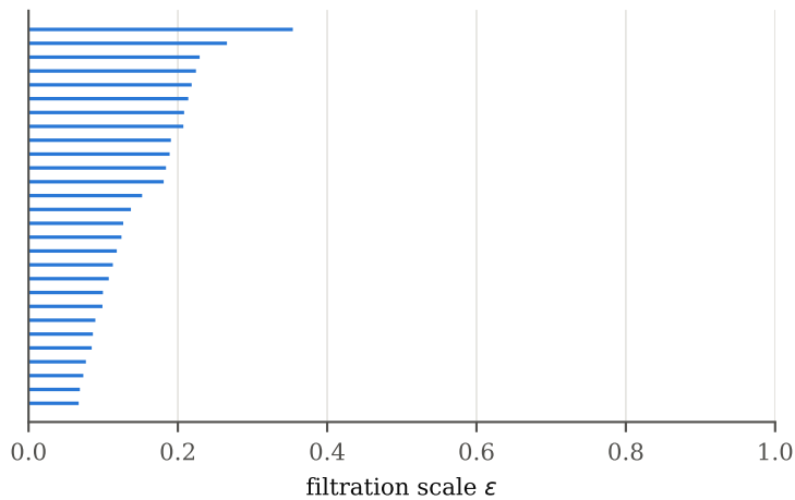
barcode: \delta_0=0.281 , P_0=12.29 , S_0=13.04 , 10 H_1 bar(s)
