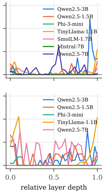
P_1 (1D total)
