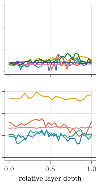
star weight S_0
