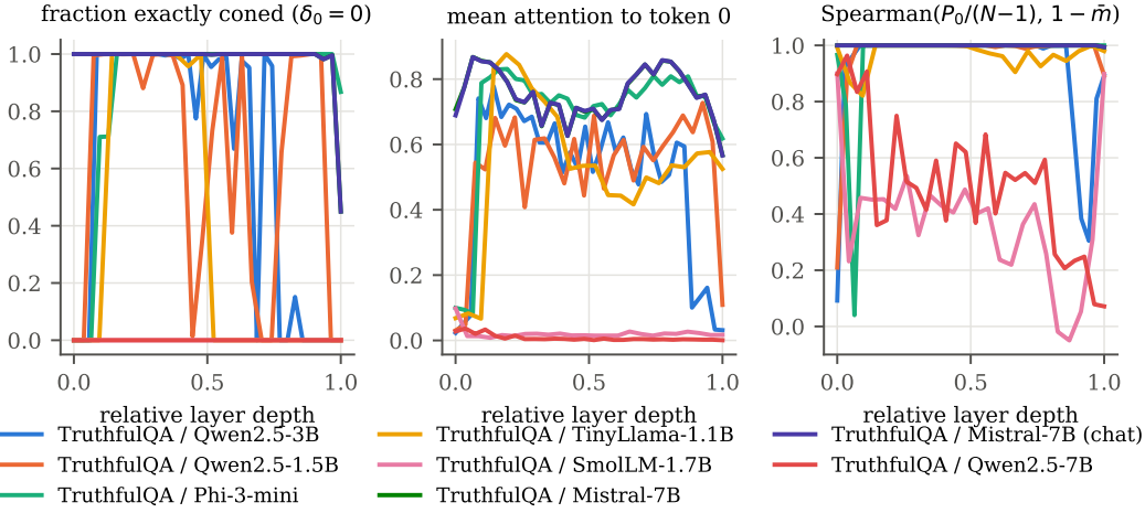
Figure 1: Layerwise structure (TruthfulQA) . Coning (left) tracks sink attention (middle); Qwen2.5-7B and SmolLM-1.7B are never coned at s = 0 . Right: length-normalized rank correlation of P_0 with sink attention, near 1 in sink models except some open layers.
