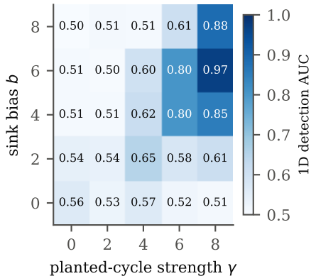
1D detects a planted cycle?
