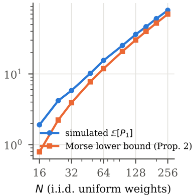
total 1D persistence
