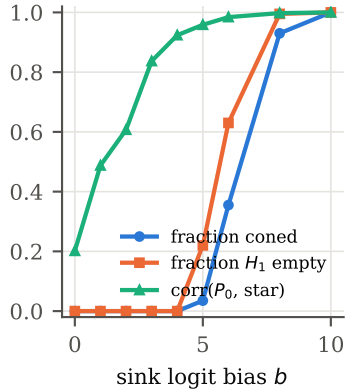
sink dose-response
