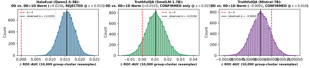
Figure 4: Paired Cluster-Bootstrap Empirical Difference Distributions. The actual 10,000-resample question-level (group) cluster-bootstrap distributions of \Delta\text{ROC-AUC} (0D vs. 0D+1D Norm.) underlying three rows of Table 3 – not illustrative placeholders. HaluEval (Qwen2.5-3B) shows a distribution clearly shifted right of zero (well-powered, non-equivalent at \epsilon=0.015 ); TruthfulQA (SmolLM-1.7B) is centered near +0.010 but wide enough to reach equivalence only at \epsilon=0.025 ; TruthfulQA (Mistral-7B) is a near-delta-function at \approx 0 , reflecting the 1D feature bank’s near-total degeneracy at this scale rather than a precisely-estimated null effect.
