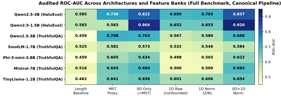
Figure 3: Audited ROC-AUC Across Architectures and Feature Banks (Canonical Pipeline). All seven settings from Table 2, including Mistral-7B and TinyLlama-1.1B. 0D persistence and combined 0D+1D features exhibit similar discriminative profiles across settings; the “0D Only (=MST)” and “MST Proxy” columns are literally the same statistic (Theorem 1) computed on different layer subsets. Mistral-7B’s 1D columns show the degenerate near-chance values discussed in §6.
