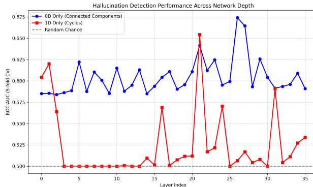
Figure 5: Layer-wise ROC-AUC across transformer depth in Qwen2.5-3B for 0D vs 1D features, visualizing Table 10.
