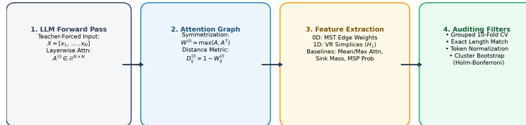
Figure 2: Auditing Pipeline. Attention matrices are symmetrized, filtered via simplicial complexes and MST, and subjected to grouped CV, synthetic controls, and equivalence testing.
