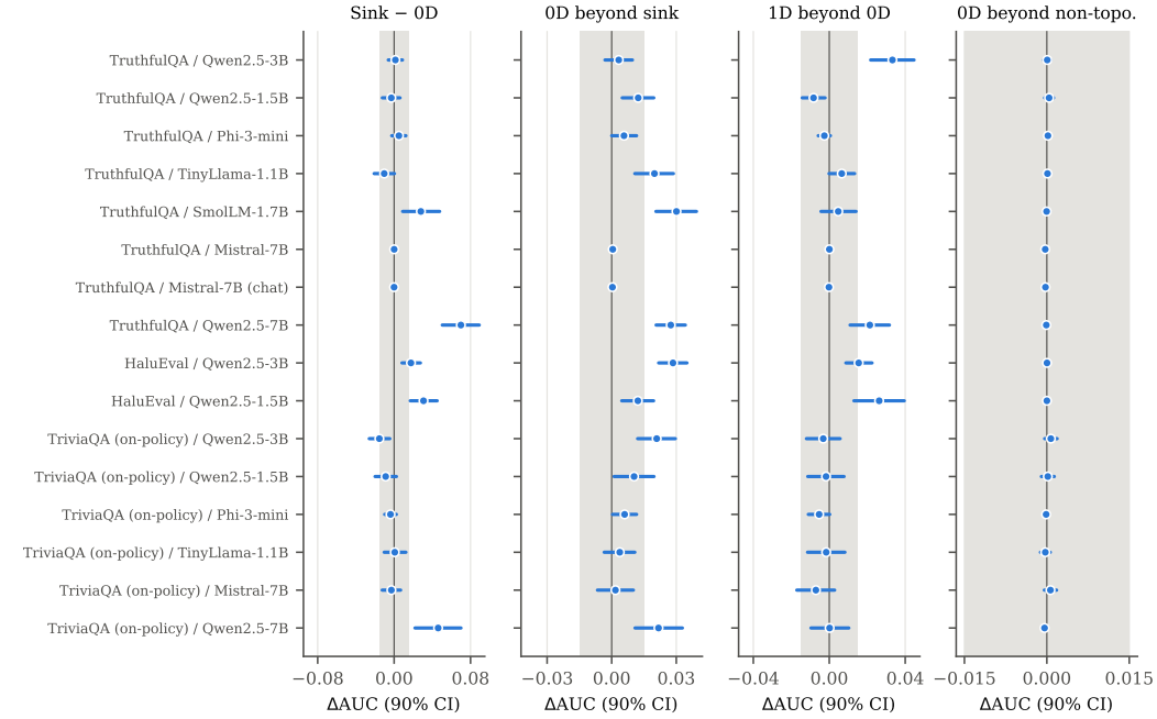
Figure 5: Four comparisons across all settings ( \Delta\text{AUC} with 90% cluster-bootstrap intervals; shaded band: \pm 0.015 ). Sink features nearly reproduce 0D; 0D adds little beyond them; 1D adds little beyond 0D except in 4 settings; and 0D adds nothing beyond non-topological probes under early fusion (late fusion in Table 20).
