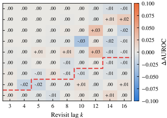
(b) Input-dependent \Delta_t minus LTI
