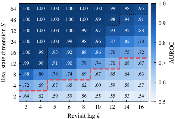
(a) LTI, learned poles: test AUROC
