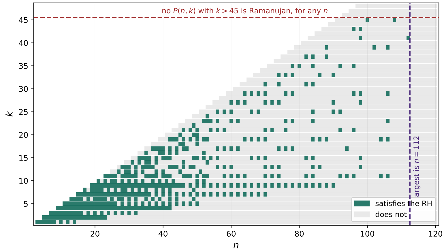
The complete classification: all 460 Ramanujan P(n, k) , decided exactly
