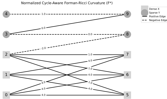
Figure 7.1. Topology of the synthetic non-homogeneous signed graph. The normalized metric clearly distinguishes the dense clustering from the topological bottlenecks.
