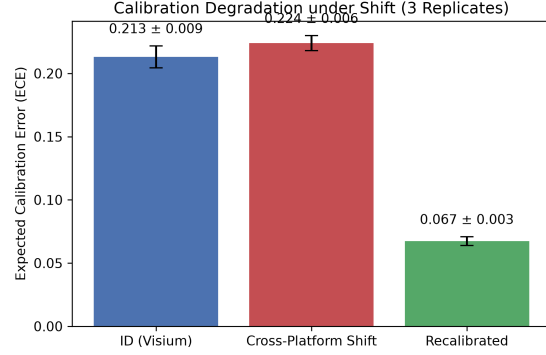
Figure 2: ECE stability across capture-rate distribution shifts. Error bars denote \pm 1 standard deviation across 3 random replicate initializations.
