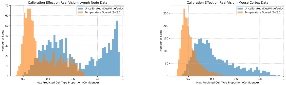
Figure 4: Qualitative confidence distributions on real spatial data (Left: Lymph Node; Right: Cortex). The uncalibrated DestVI model produces highly uncalibrated predictions, which are effectively smoothed to biologically plausible profiles by Temperature Scaling.
