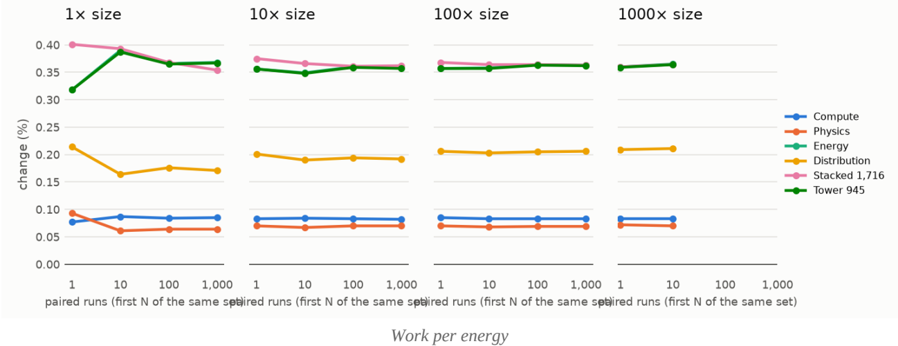
Six organisms: work per energy, Omni against native (model)
