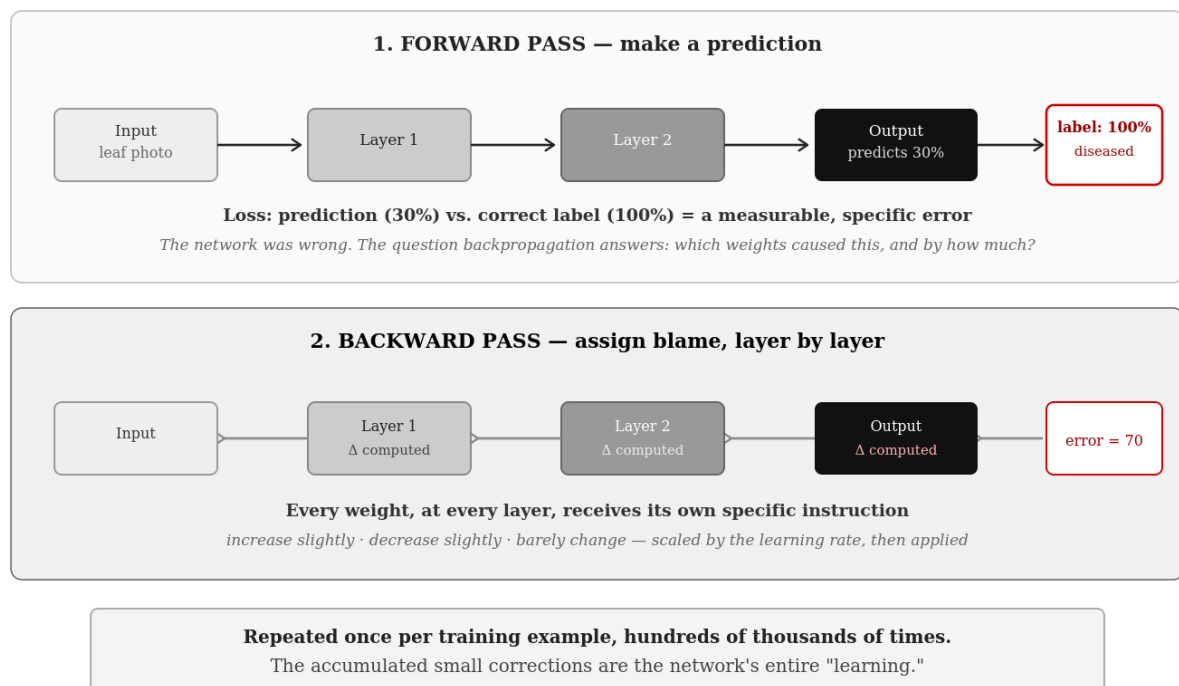
Figure 7.7 — How Backpropagation Works
