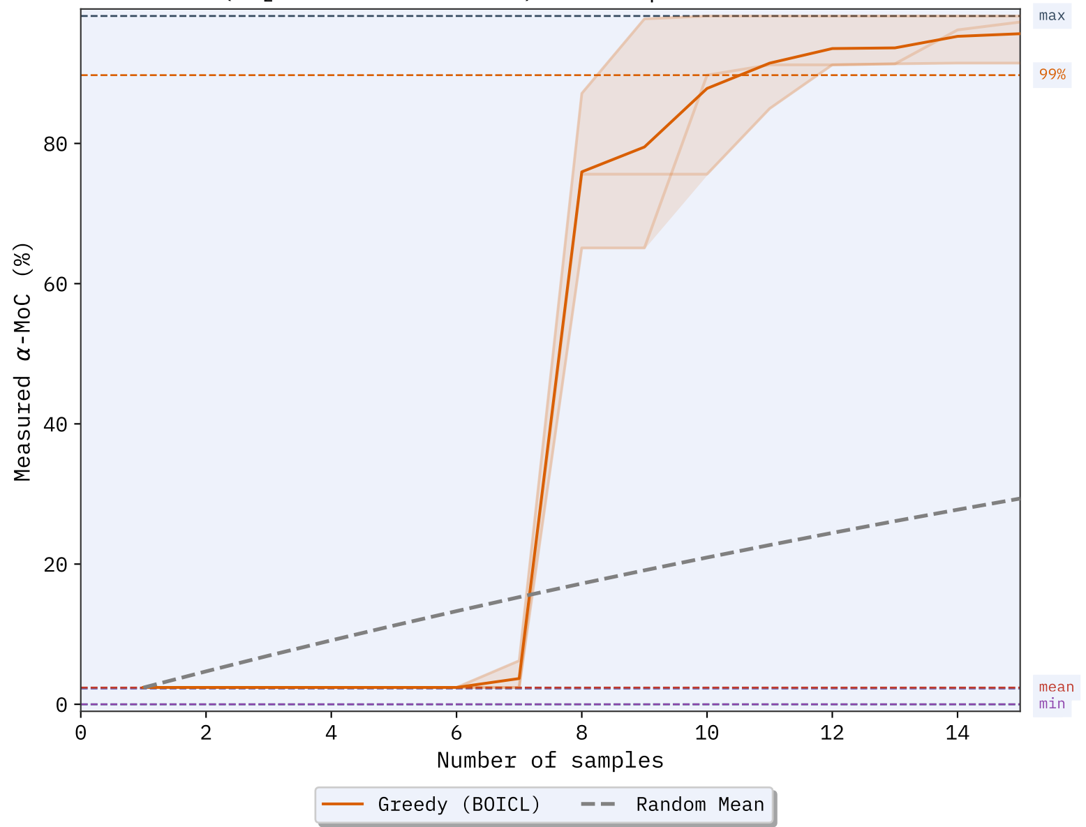
GPT-4o (Mo 2 C \alpha -MoC isolation) — 3 replicates vs Random Mean
