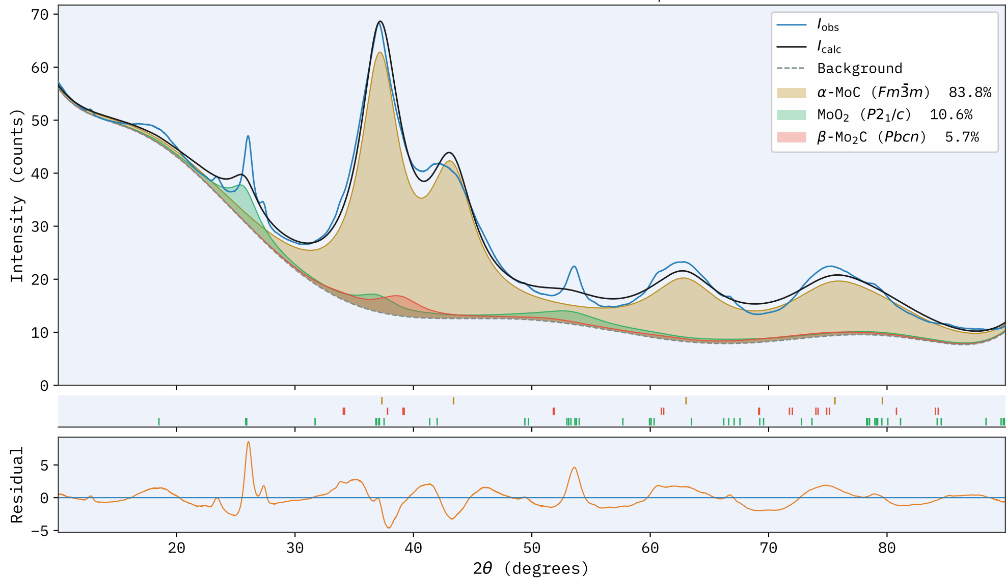
GSAS-II Rietveld refinement — R_{wp} = 5.72\%
